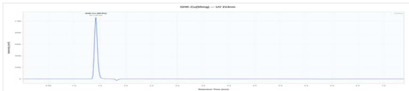
GHK-Cu 50mg - 2026-001: UV Chromatogram
